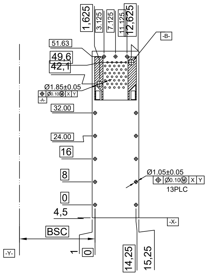
ECOMMENDED PCB CONFIGURATION
