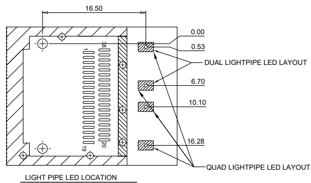
LIGHT PIPE LED LOCATION
