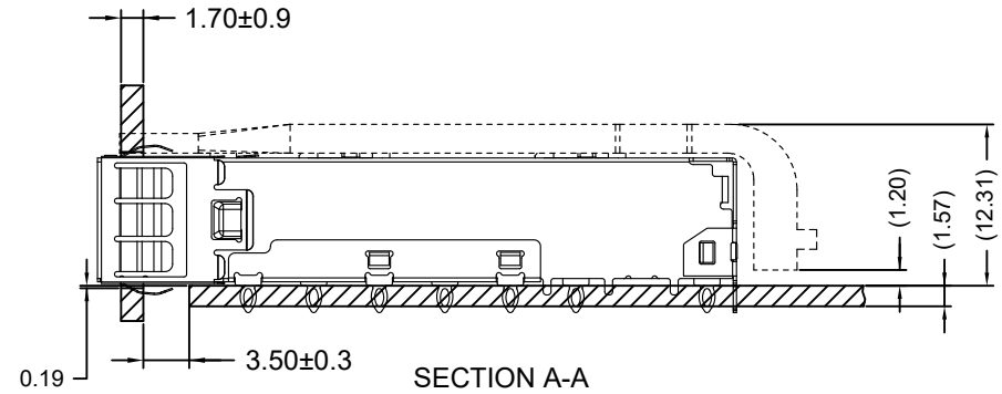
RECOMMENDED BEZEL DESIGN
