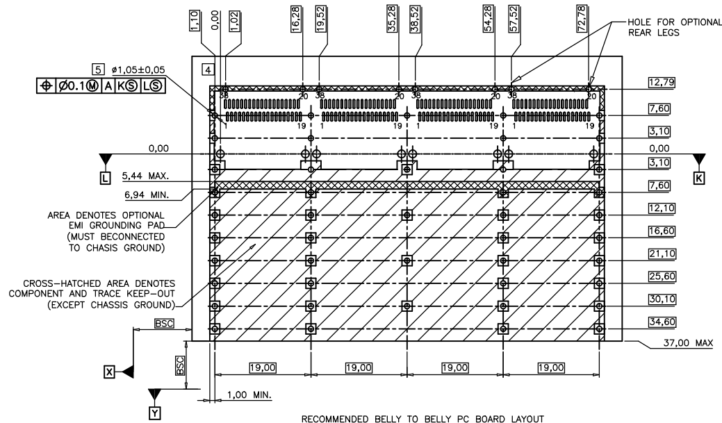
RECOMMENDED BELLY TO BELLY PC BOARD LAYOUT
