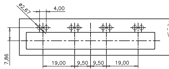
BEZEL L/P CUT-OUT POSITION DIMENSION FOR SINGLE SIDE MOUNTING (SPRING FINGER)
