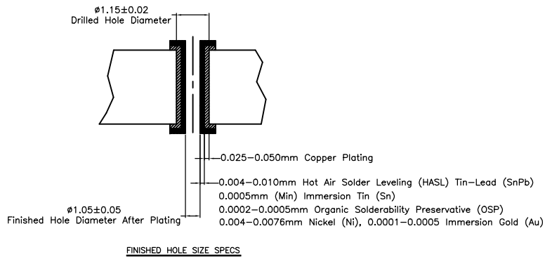
FINISHED HOLE SIZE SPECS
