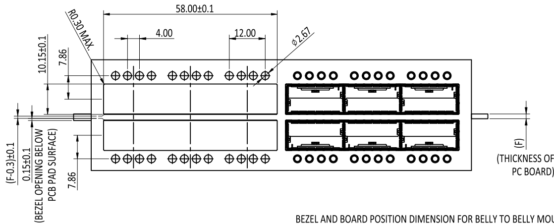
BEZEL AND BOARD POSITION DIMENSION FOR BELLY TO BELLY MOUNTING
