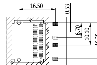
QUAD LIGHT PIPE LED LOCATION
