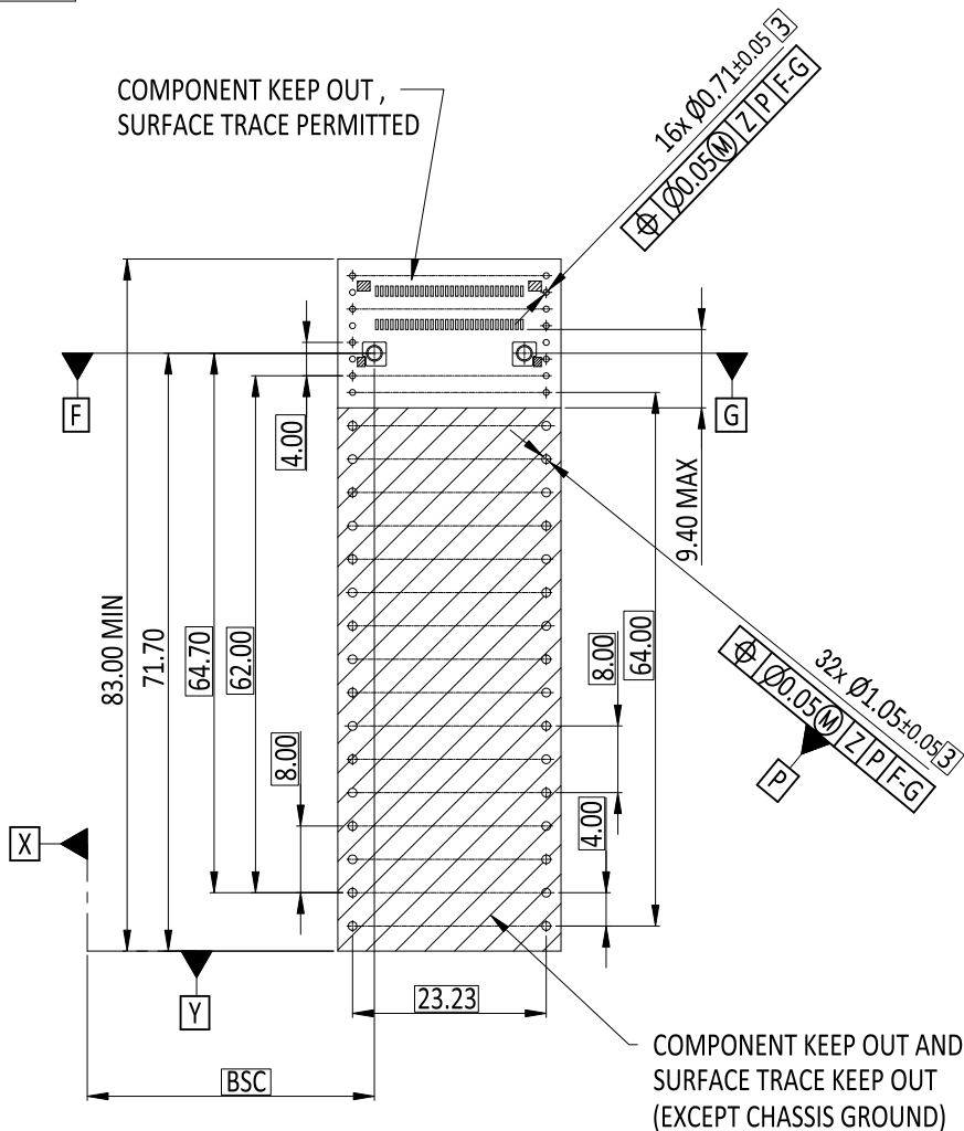
RECOMMENDED BELLY TO BELLY PC BOARD LAYOUT
