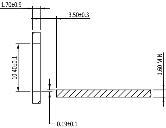
BEZEL OPENING BELOW PC BOARD
