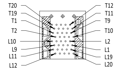
CONNECTOR PIN-OUT COMPONENT SIDE OF BOARD
