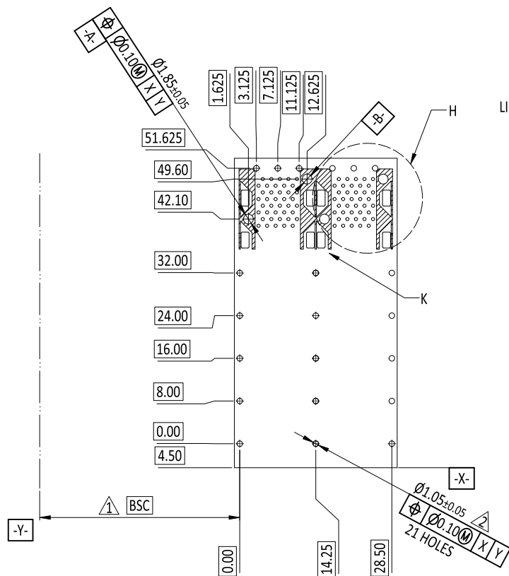
RECOMMENDED PCB CONFIGURATION
