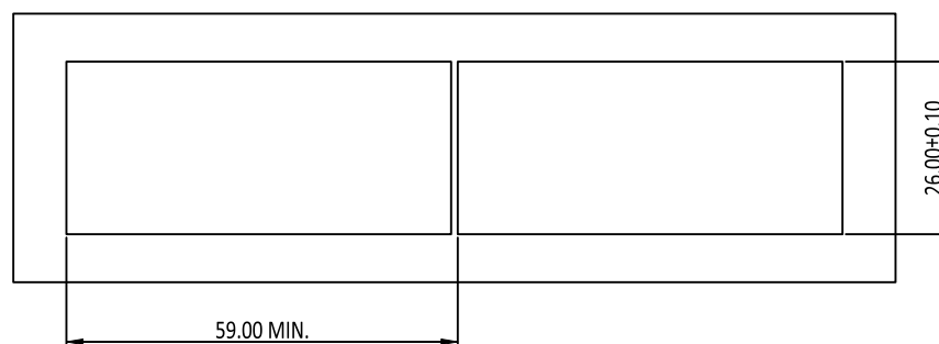
RECOMMENDED BEZEL DESIGN
