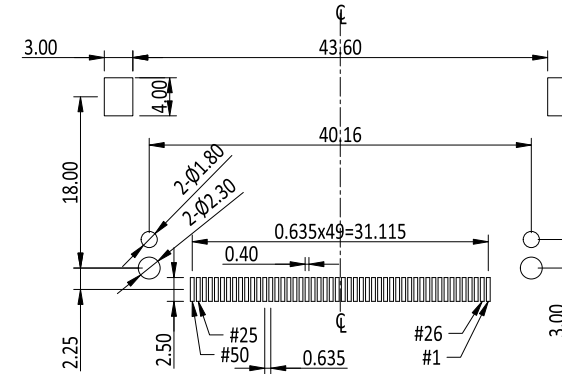
RECOMMENDED P.C.B LAYOUT TOLERANCES: ±0.05mm
