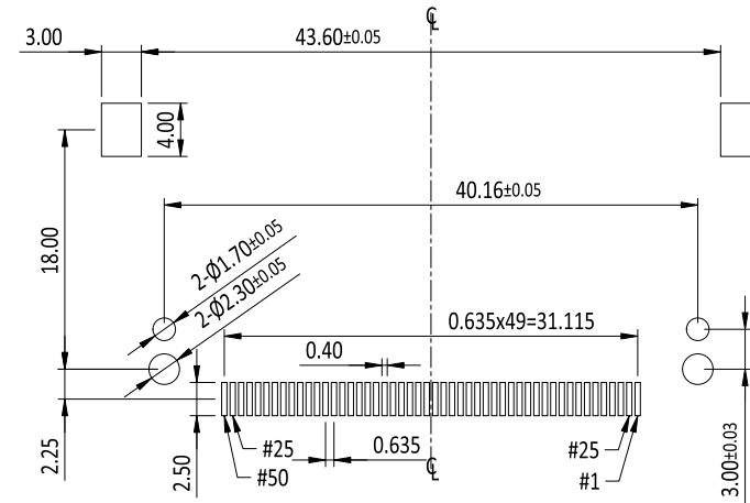
RECOMMENDED P.C.B LAYOUT TOLERANCES: ±0.05mm
