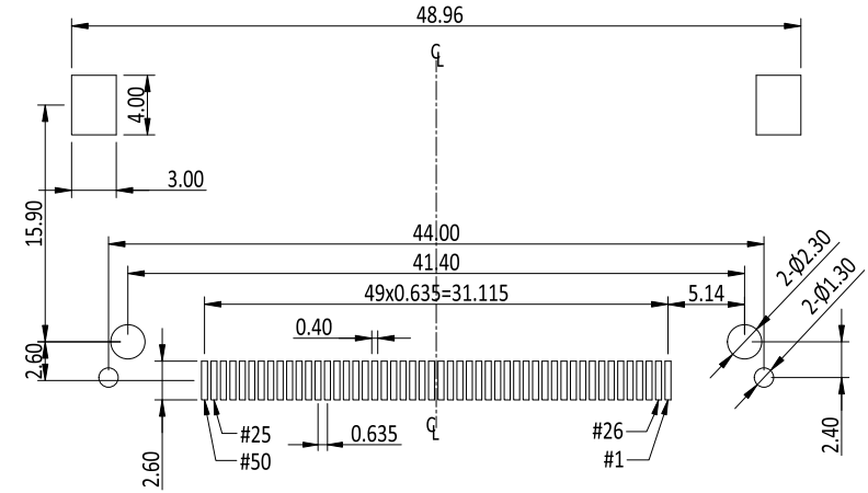
RECOMMENDED P.C.B LAYOUT TOLERANCES: ±0.05mm
