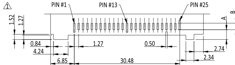
RECOMMENDED P.C.B LAYOUT (TOP VIEW) TOLERANCES: ±0.05mm (PCB THK=0.5mm)
