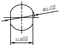
Recommended Panel Cut- Out
