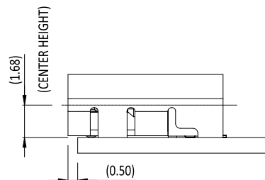
MATING CONDITION
