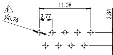
RECOMMENDED PCB LAYOUT (TOP VIEW) TOLERANCES: ±0.05mm
