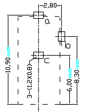
Recommend PCB Layout PCB Top View
