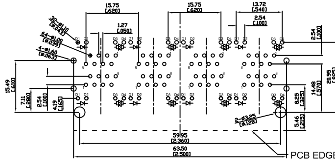
RECOMMENDED PCB LAYOUT TOP VIEW TOLERANCE: ±0.05mm PCB THICKNESS: 1.60±0.05mm
