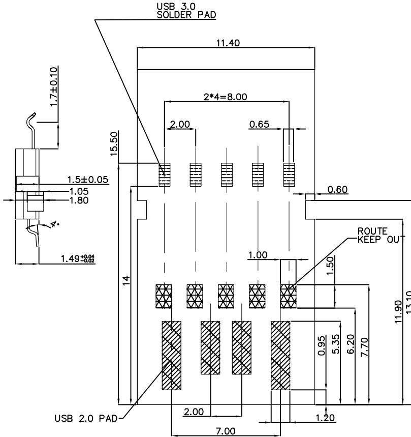
RECOMMENDED P.C.B LAYOUT GENERAL TOLERANCE : ±0.05mm
