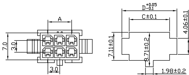
PANEL OPENING
