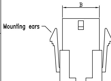
TYPE 2 W/Latch
