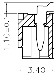
SECTION E-E
