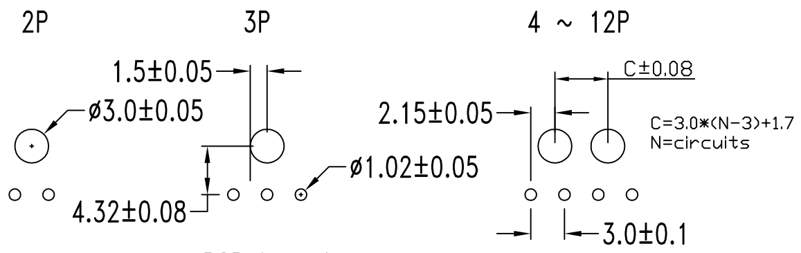
PCB Layout
