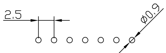
P. C. board hole dimensions
