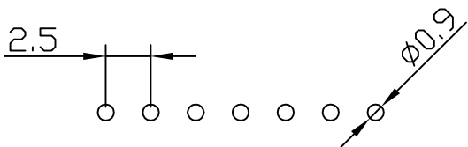
P. C. board hole dimensions
