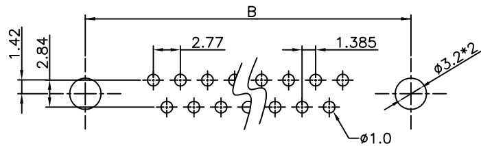
RECOMMENDED P.C.B LAYOUT (TOP VIEW) TOLERANCES: \pm 0.05\text{mm}
