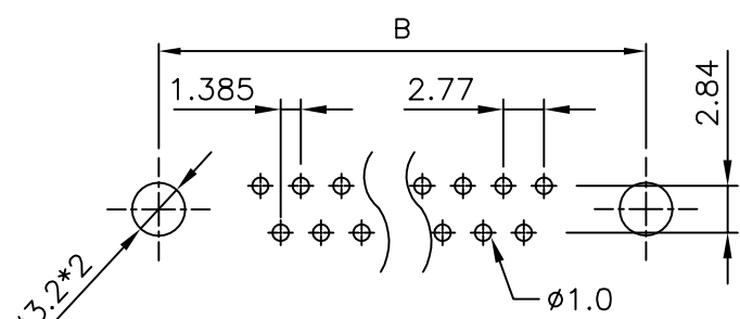
RECOMMENDED P.C.B LAYOUT (TOP VIEW) TOLERANCES: ±0.05mm
