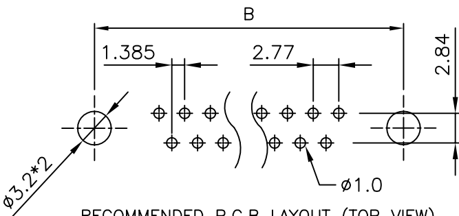
RECOMMENDED P.C.B LAYOUT (TOP VIEW) TOLERANCES: ±0.05mm
