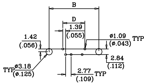
P.C.B LAYOUT TOLERANCES: ±0.05mm
