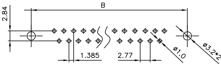
RECOMMENDED P.C.B. LAYOUT(TOP VIEW) TOLERANCES:±0.05mm
