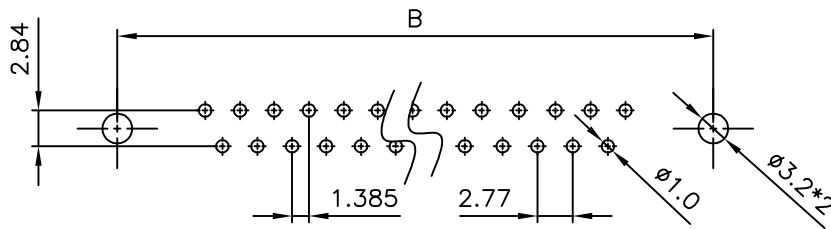
RECOMMENDED P.C.B. LAYOUT(TOP VIEW) TOLERANCES:±0.05mm
