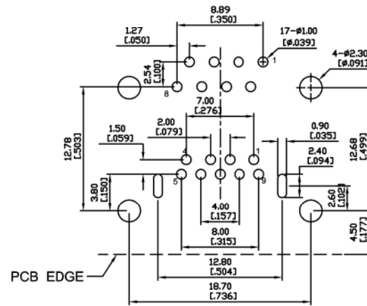
RECOMMENDED PCB LAYOUT TOP VIEW TOLERANCE: ±0.05mm PCB THICKNESS: 1.60±0.05mm
