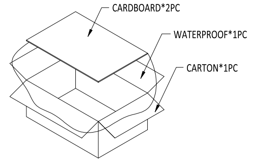
(CARTON: L457xW298xH228mm, MATERIAL K=K)
