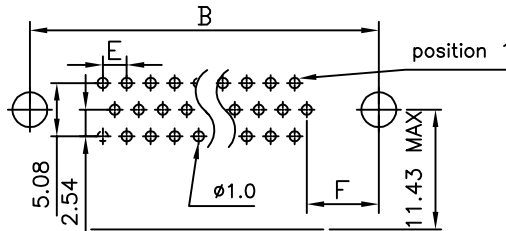
EDGE OF P.C.B. BOARD RECOMMENDED P.C.B. LAYOUT (TOP VIEW) TOLERANCES: ±0.05mm
